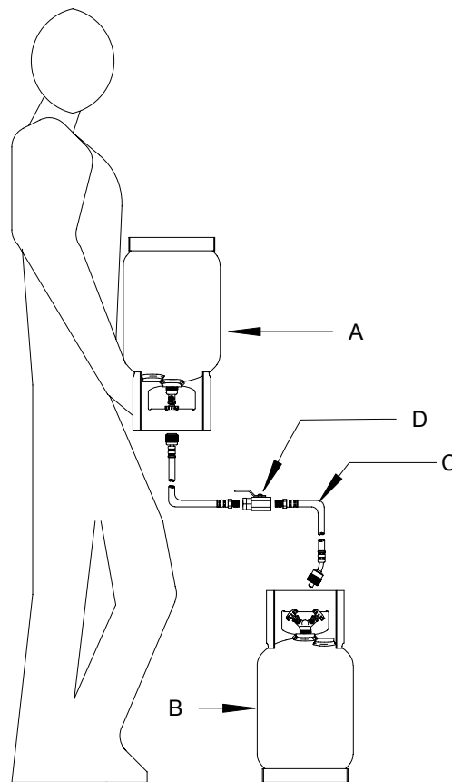
FIGURE 6 CHARGING TANK
