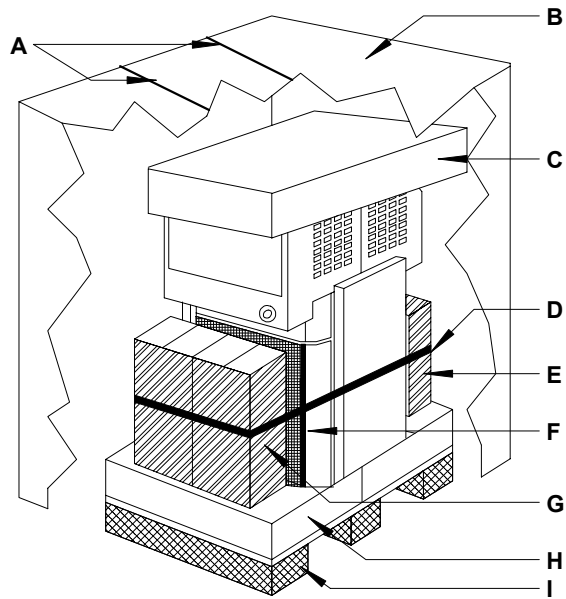
FIGURE 1 Unit Package
