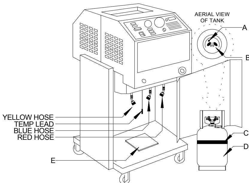
FIGURE 5 TANK INSTALLATION
